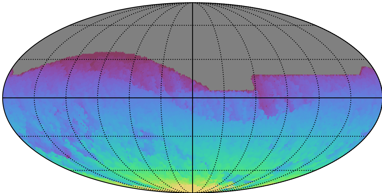
roll_pause_mjdp365_v3.4_10yrs All sky all bands: Max HA
