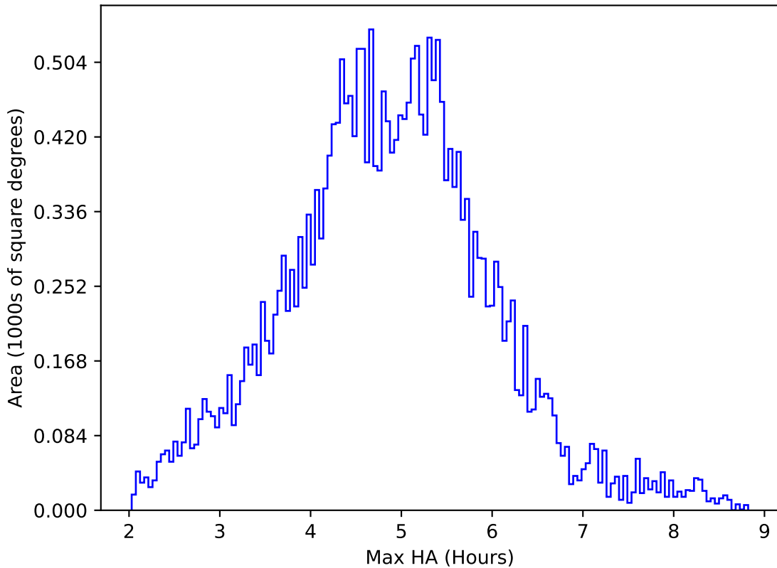
roll_pause_mjdp365_v3.4_10yrs All sky all bands: Max HA
