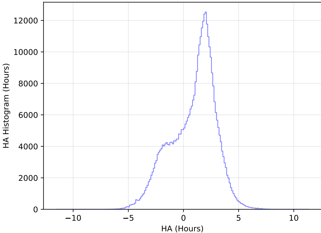
roll_pause_mjdp365_v3.4_10yrs WFD y band: HA Histogram
