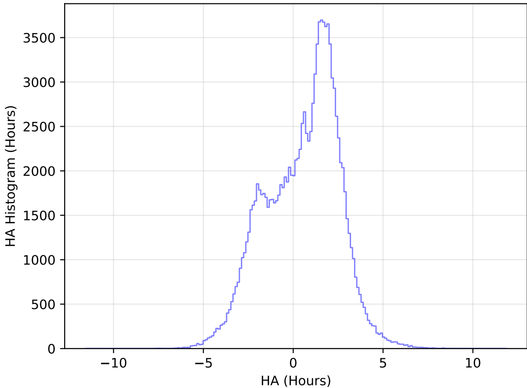
roll_pause_mjdp365_v3.4_10yrs WFD u band: HA Histogram
