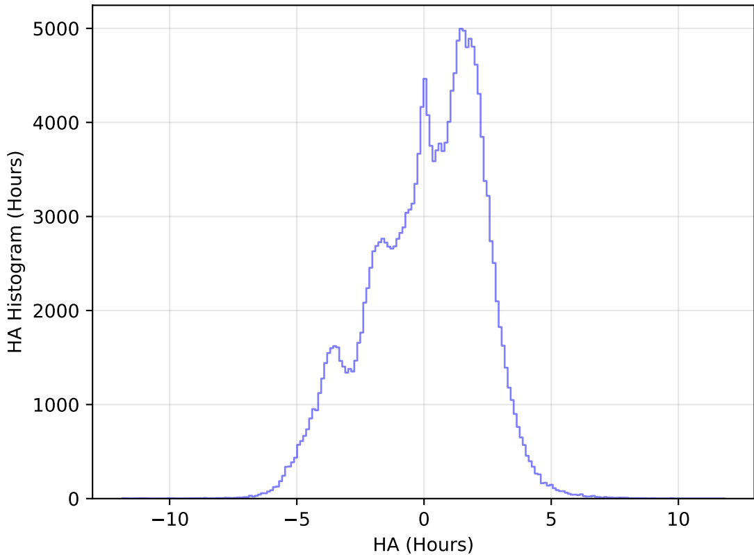
roll_pause_mjdp365_v3.4_10yrs WFD g band: HA Histogram
