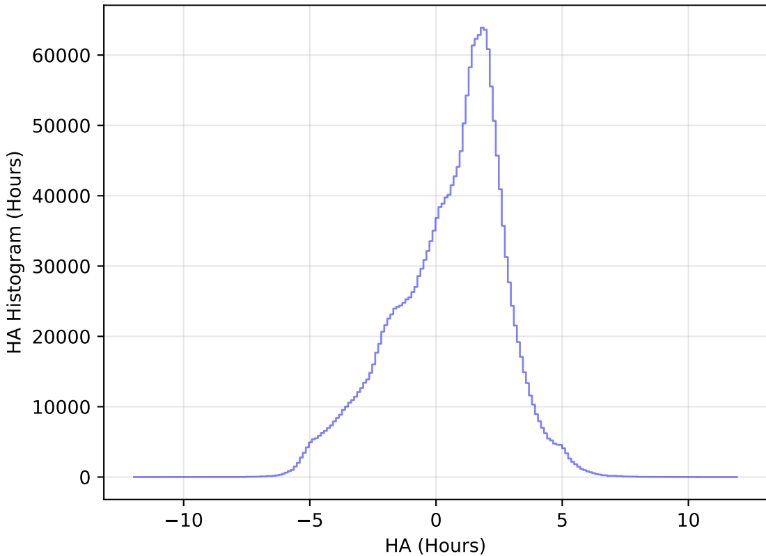
roll_pause_mjdp365_v3.4_10yrs WFD all bands: HA Histogram
