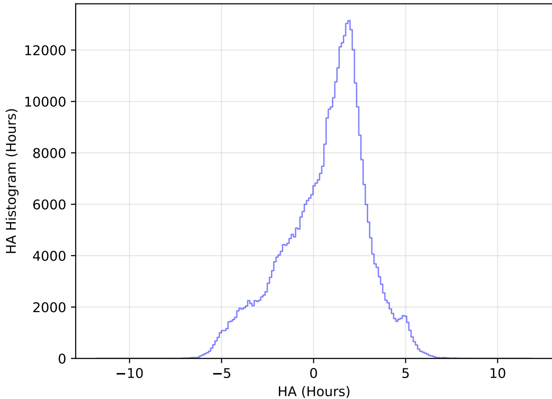
roll_pause_mjdp365_v3.4_10yrs All sky z band: HA Histogram
