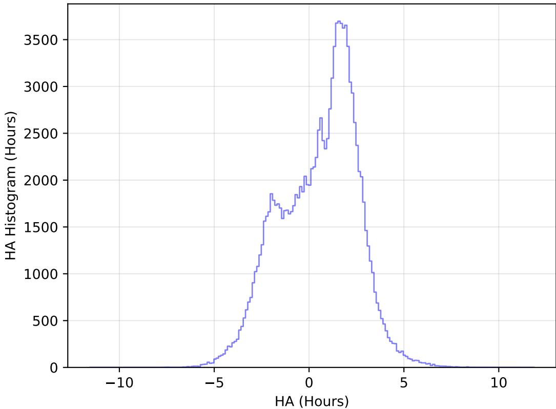
roll_pause_mjdp365_v3.4_10yrs All sky u band: HA Histogram
