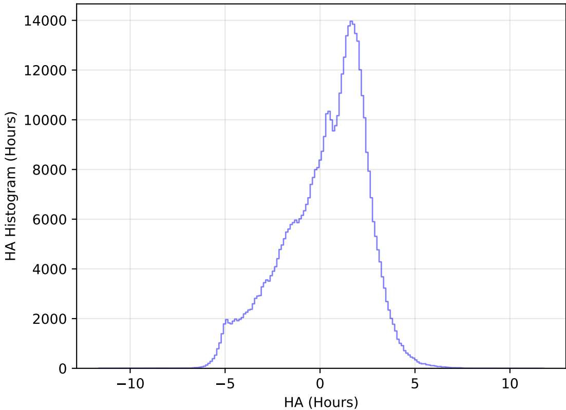
roll_pause_mjdp365_v3.4_10yrs All sky r band: HA Histogram
