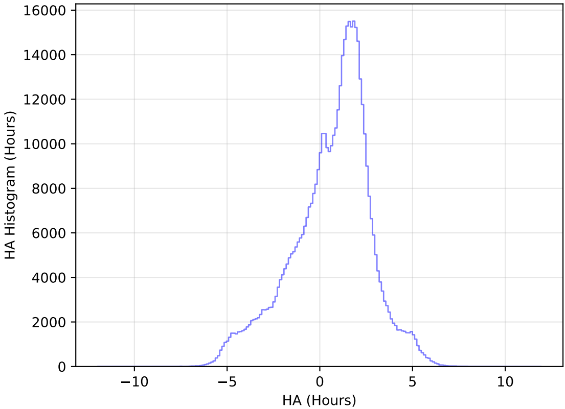
roll_pause_mjdp365_v3.4_10yrs All sky i band: HA Histogram
