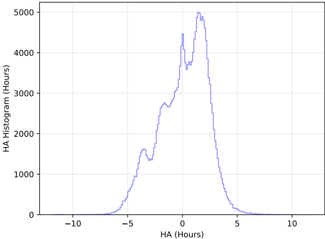
roll_pause_mjdp365_v3.4_10yrs All sky g band: HA Histogram
