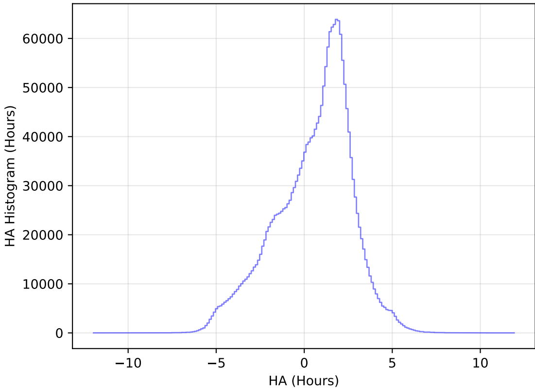
roll_pause_mjdp365_v3.4_10yrs All sky all bands: HA Histogram
