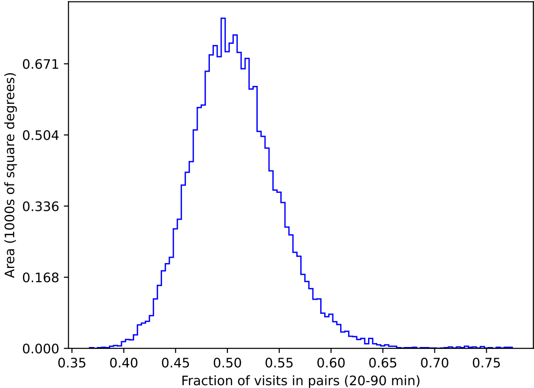
roll_pause_mjdp365_v3.4_10yrs gri WFD: Fraction of visits in pairs (20-90 min)
