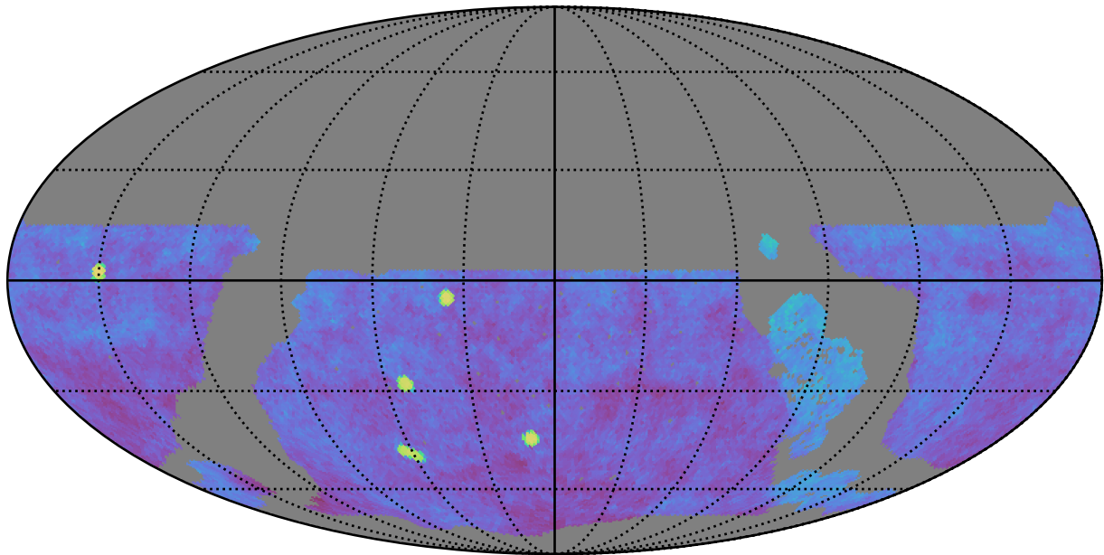
roll_pause_mjdp365_v3.4_10yrs gri WFD: Fraction of visits in pairs (10-60 min)
