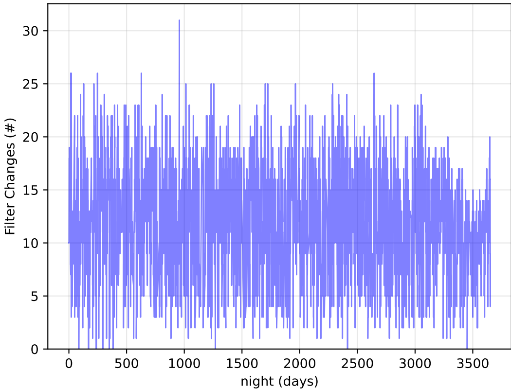
roll_pause_mjdp365_v3.4_10yrs Per Night: Filter Changes
