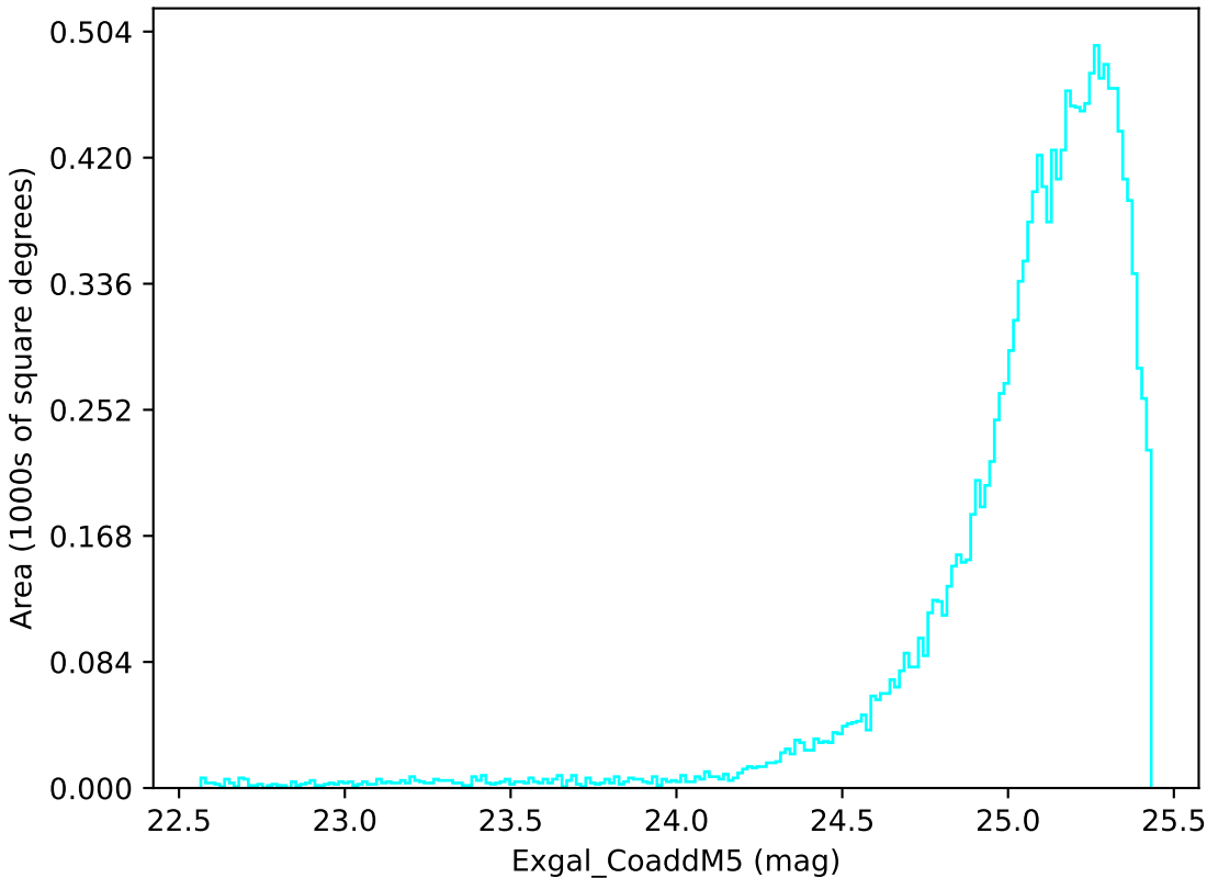
roll_pause_mjdp365_v3.4_10yrs WFD u band: Exgal_CoaddM5
