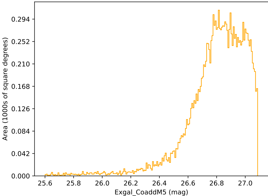
roll_pause_mjdp365_v3.4_10yrs WFD r band: Exgal_CoaddM5
