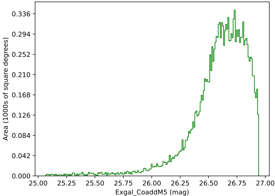
roll_pause_mjdp365_v3.4_10yrs WFD g band: Exgal_CoaddM5
