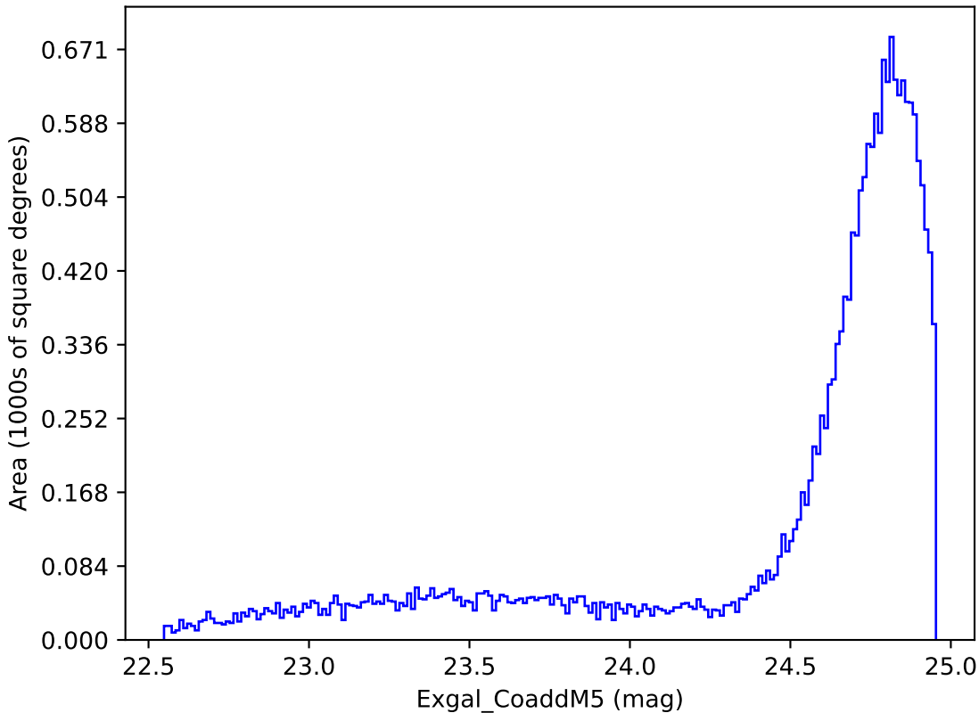
roll_pause_mjdp365_v3.4_10yrs All sky y band: Exgal_CoaddM5
