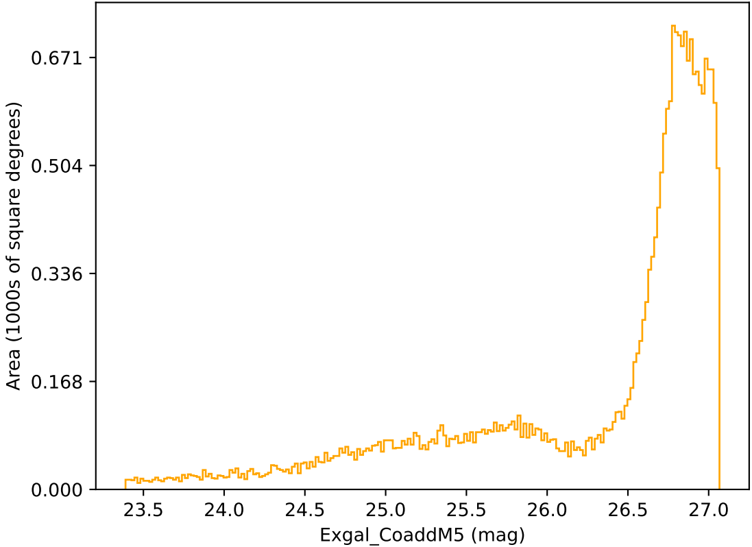
roll_pause_mjdp365_v3.4_10yrs All sky r band: Exgal_CoaddM5
