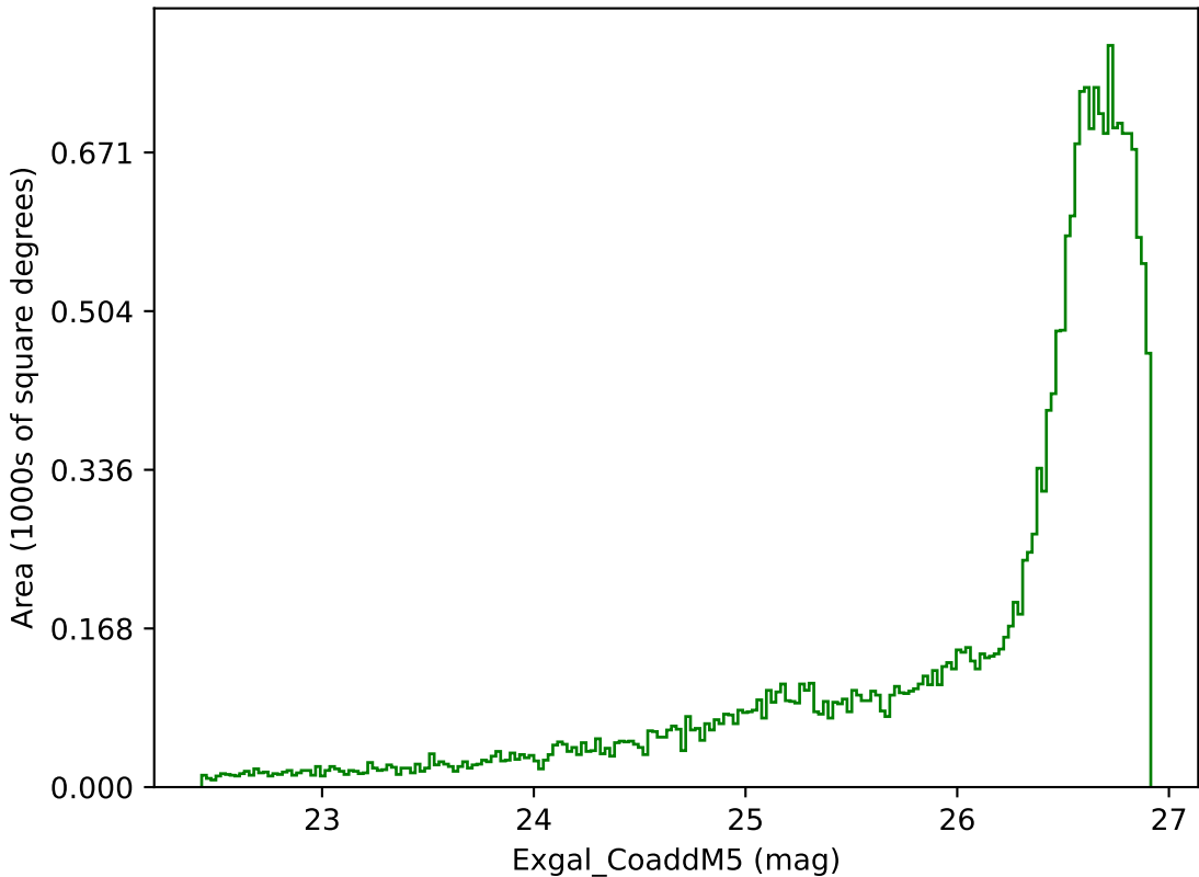
roll_pause_mjdp365_v3.4_10yrs All sky g band: Exgal_CoaddM5
