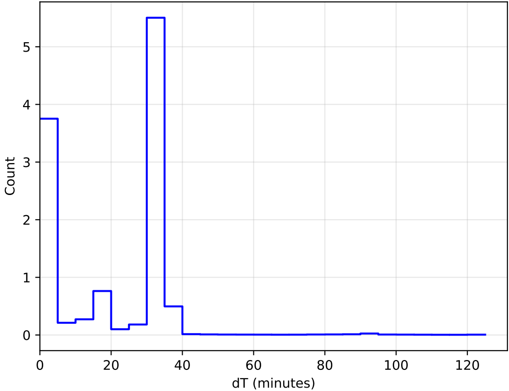
roll_pause_mjdp365_v3.4_10yrs WFD: DeltaT Histogram
