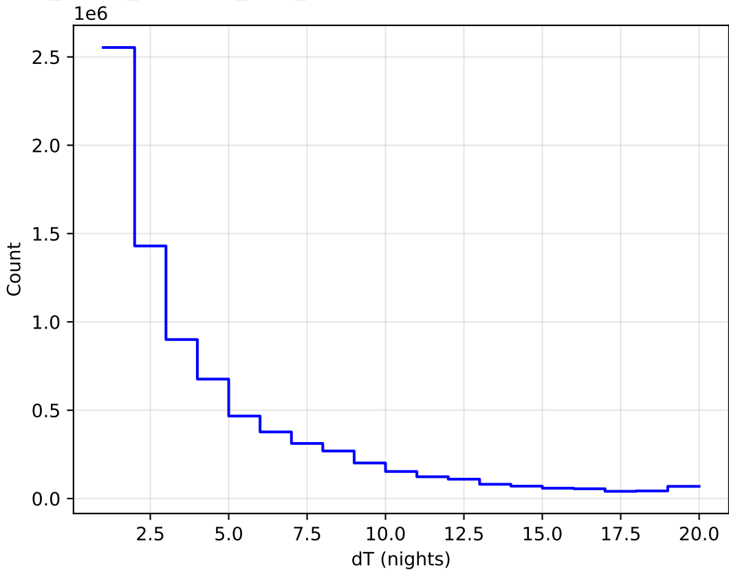
roll_pause_mjdp365_v3.4_10yrs WFD all bands: DeltaNight Histogram
