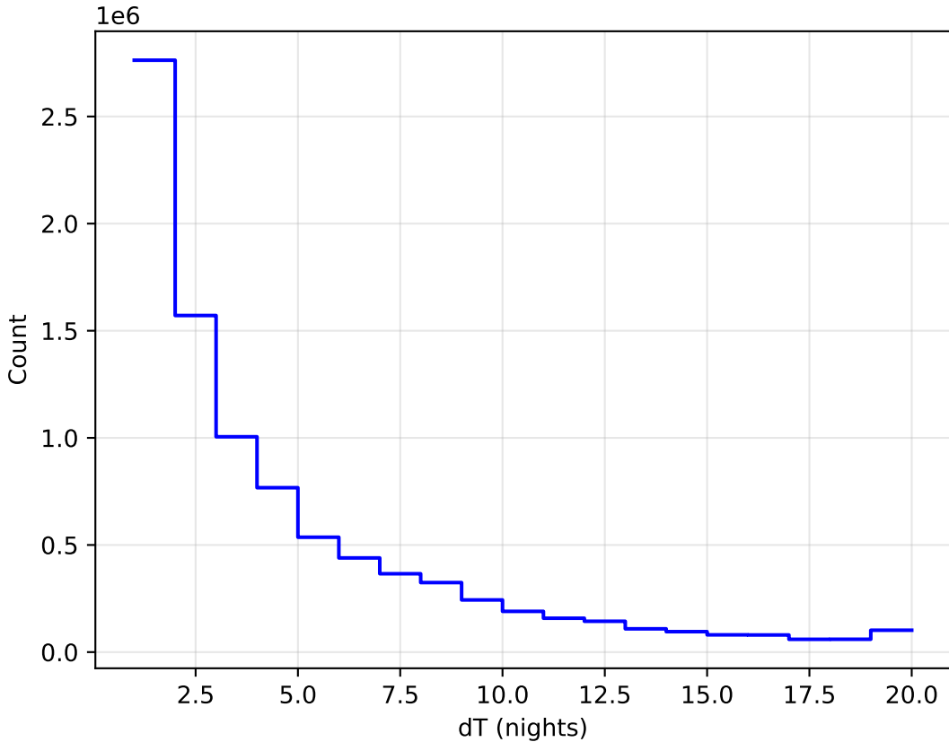
roll_pause_mjdp365_v3.4_10yrs All sky all bands: DeltaNight Histogram
