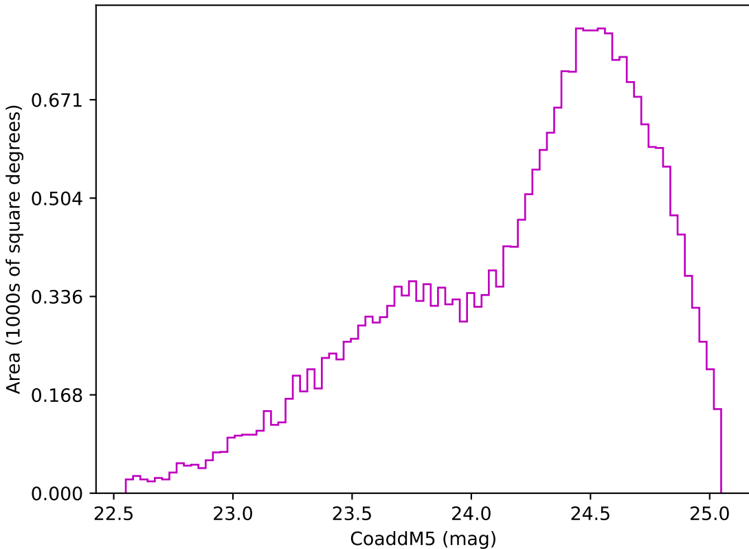
roll_pause_mjdp365_v3.4_10yrs Yr 3-4 z band: CoaddM5
