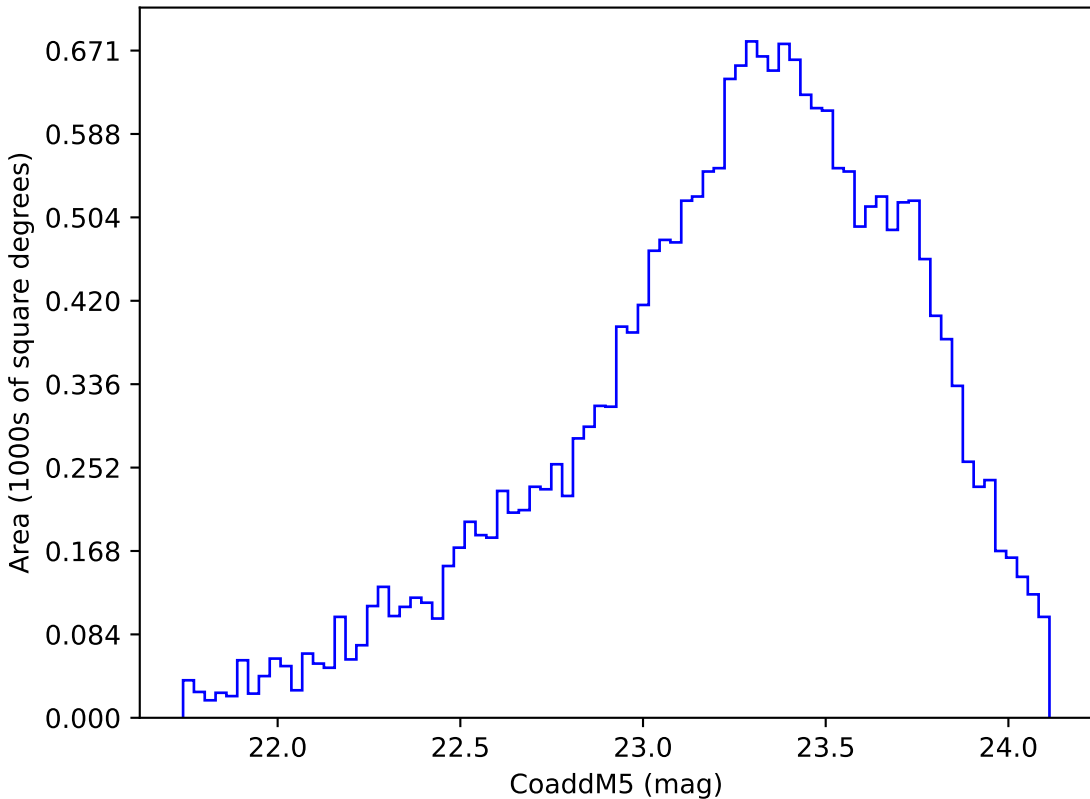
roll_pause_mjdp365_v3.4_10yrs Yr 3-4 y band: CoaddM5
