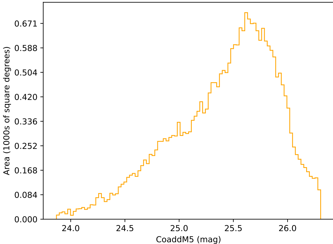
roll_pause_mjdp365_v3.4_10yrs Yr 3-4 r band: CoaddM5
