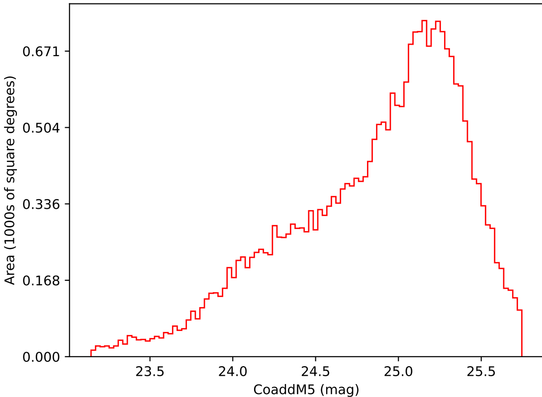
roll_pause_mjdp365_v3.4_10yrs Yr 3-4 i band: CoaddM5
