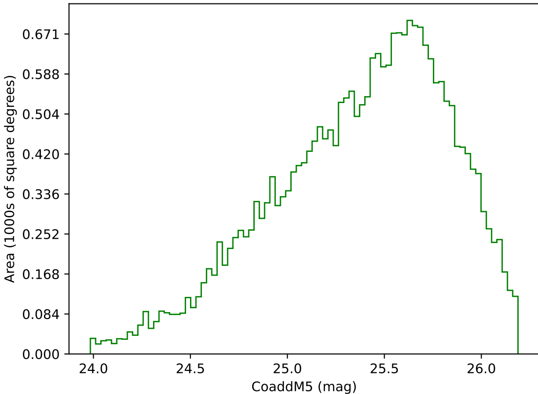
roll_pause_mjdp365_v3.4_10yrs Yr 3-4 g band: CoaddM5
