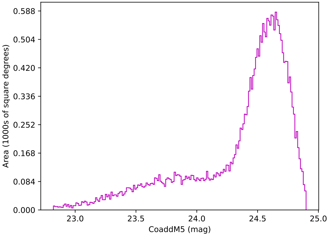
roll_pause_mjdp365_v3.4_10yrs Yr 1 z band: CoaddM5
