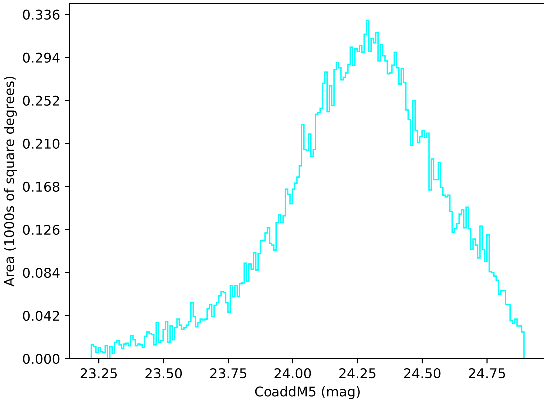
roll_pause_mjdp365_v3.4_10yrs Yr 1 u band: CoaddM5
