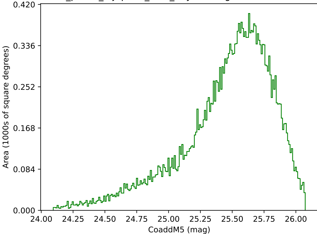
roll_pause_mjdp365_v3.4_10yrs Yr 1 g band: CoaddM5
