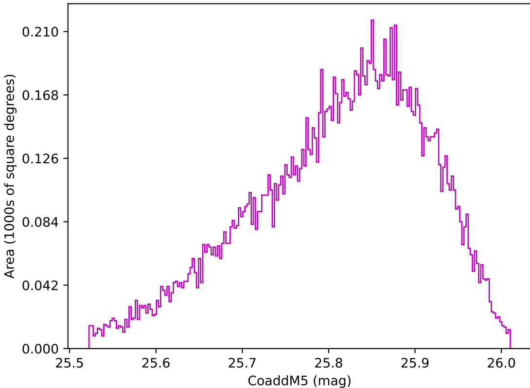
roll_pause_mjdp365_v3.4_10yrs WFD z band: CoaddM5
