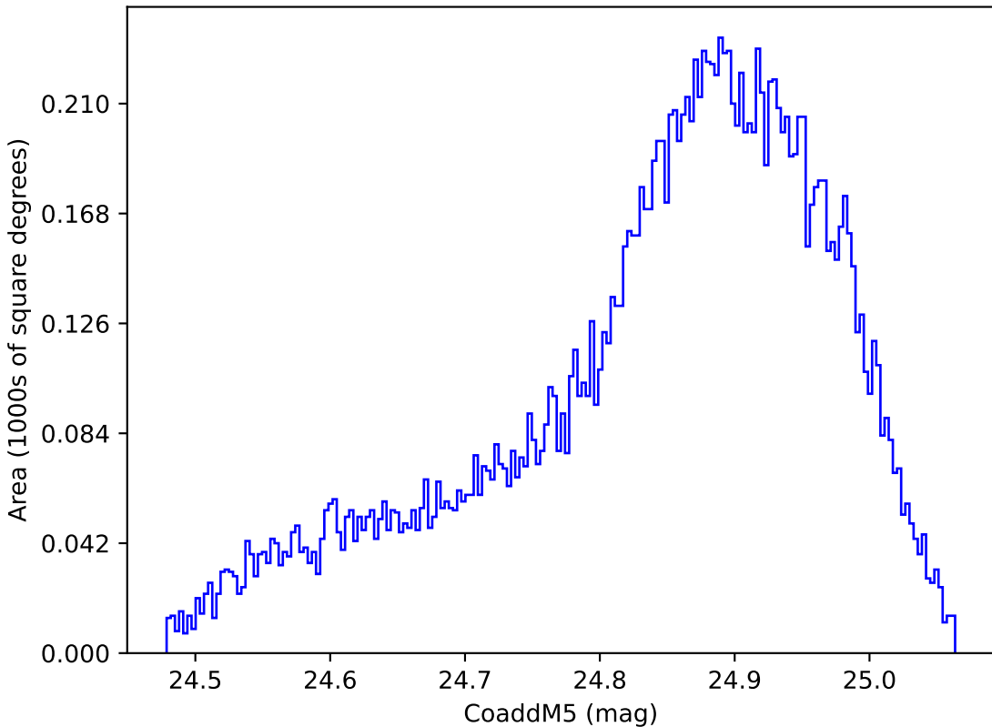
roll_pause_mjdp365_v3.4_10yrs WFD y band: CoaddM5
