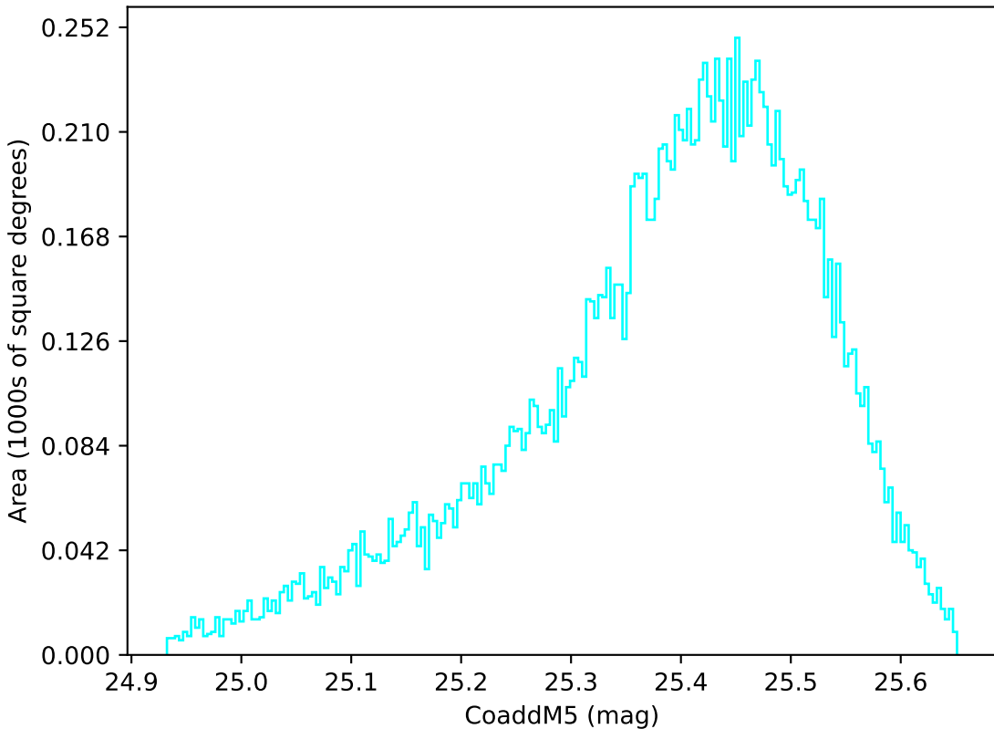
roll_pause_mjdp365_v3.4_10yrs WFD u band: CoaddM5
