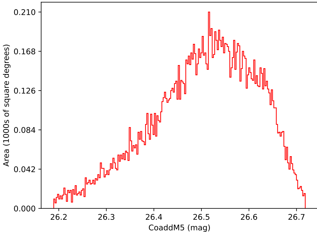
roll_pause_mjdp365_v3.4_10yrs WFD i band: CoaddM5
