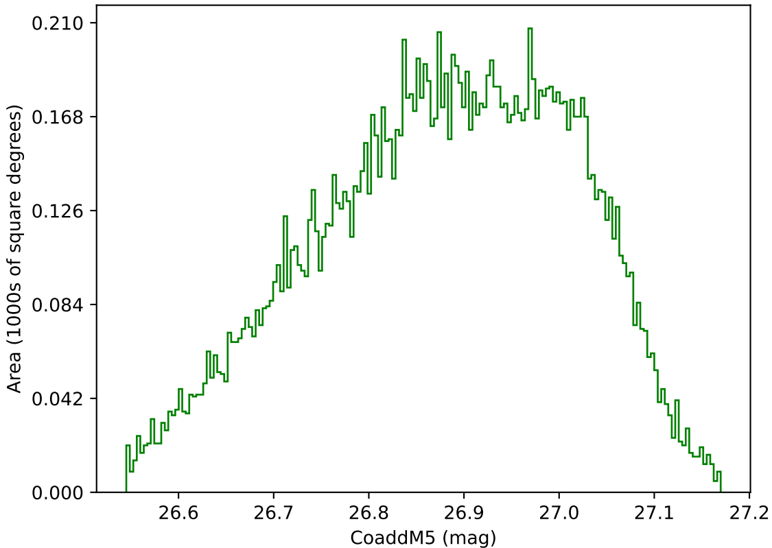
roll_pause_mjdp365_v3.4_10yrs WFD g band: CoaddM5
