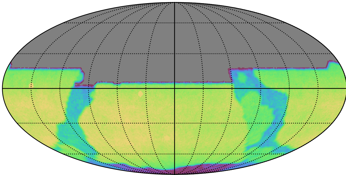
roll_pause_mjdp365_v3.4_10yrs All sky y band: CoaddM5
