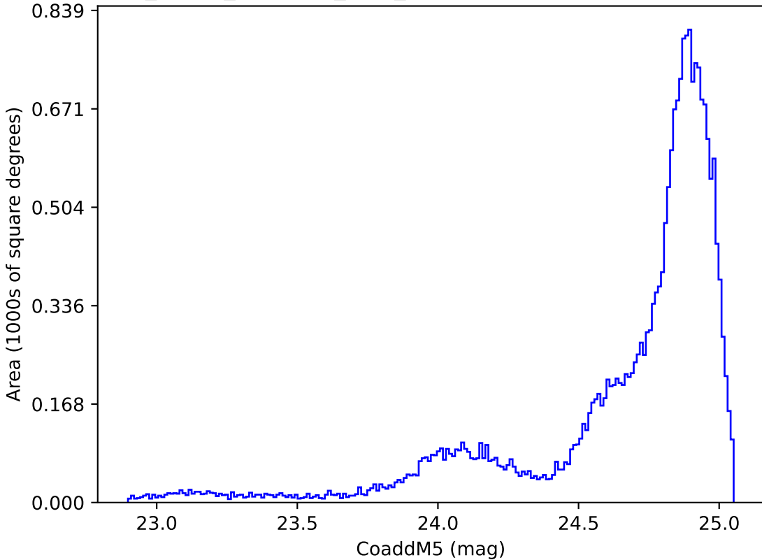
roll_pause_mjdp365_v3.4_10yrs All sky y band: CoaddM5
