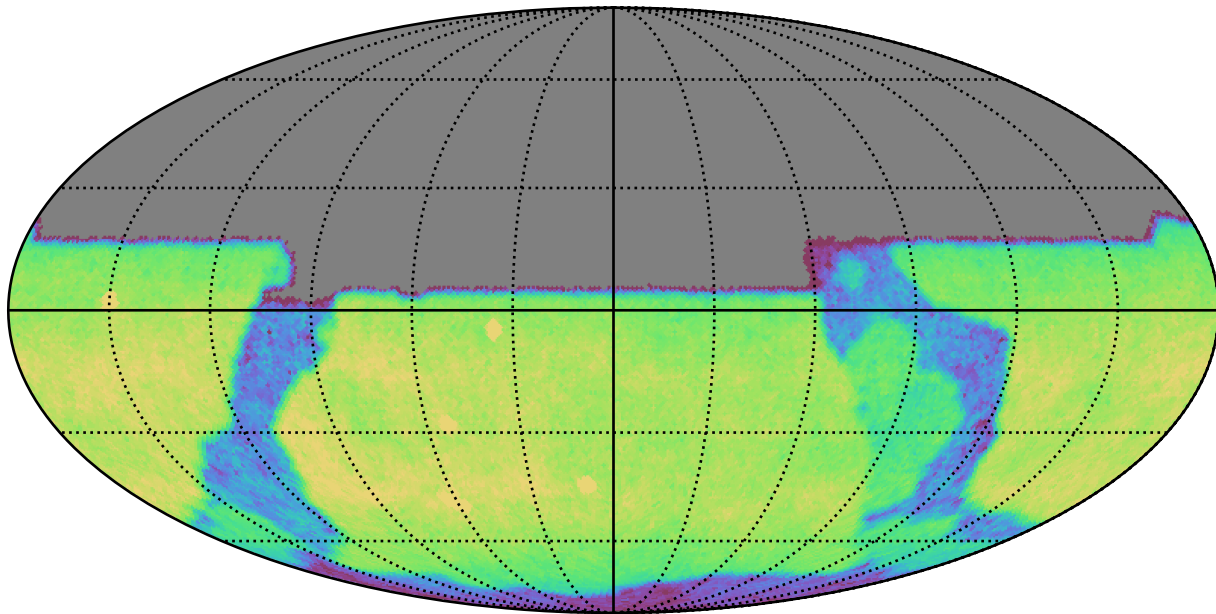
roll_pause_mjdp365_v3.4_10yrs All sky u band: CoaddM5
