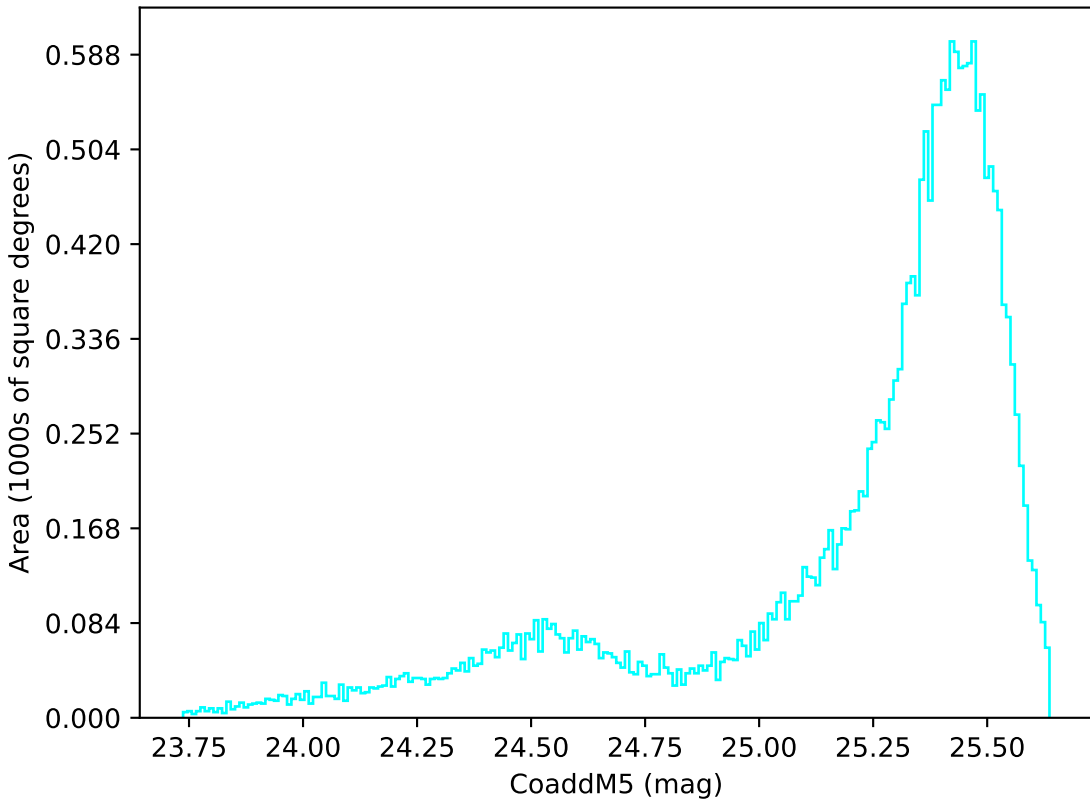
roll_pause_mjdp365_v3.4_10yrs All sky u band: CoaddM5
