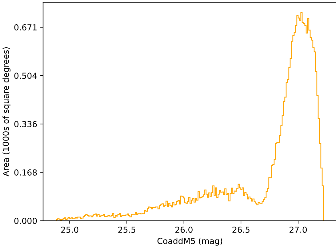
roll_pause_mjdp365_v3.4_10yrs All sky r band: CoaddM5
