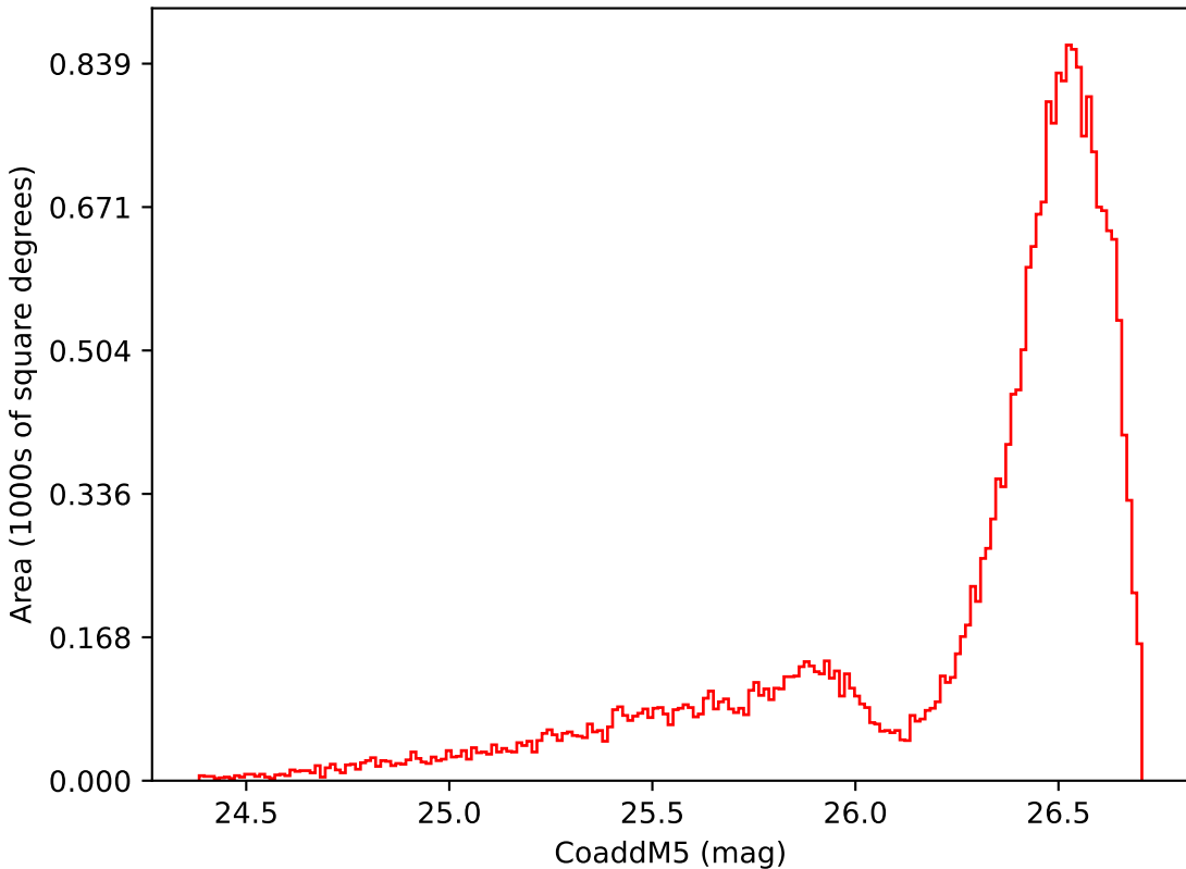
roll_pause_mjdp365_v3.4_10yrs All sky i band: CoaddM5
