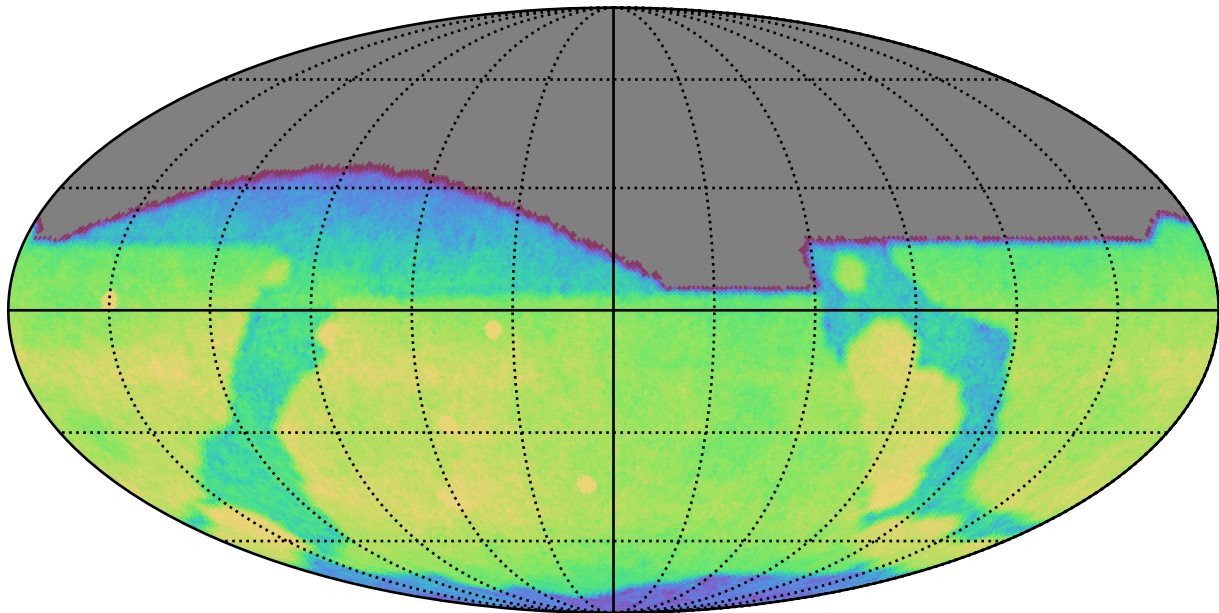
roll_pause_mjdp365_v3.4_10yrs All sky g band: CoaddM5
