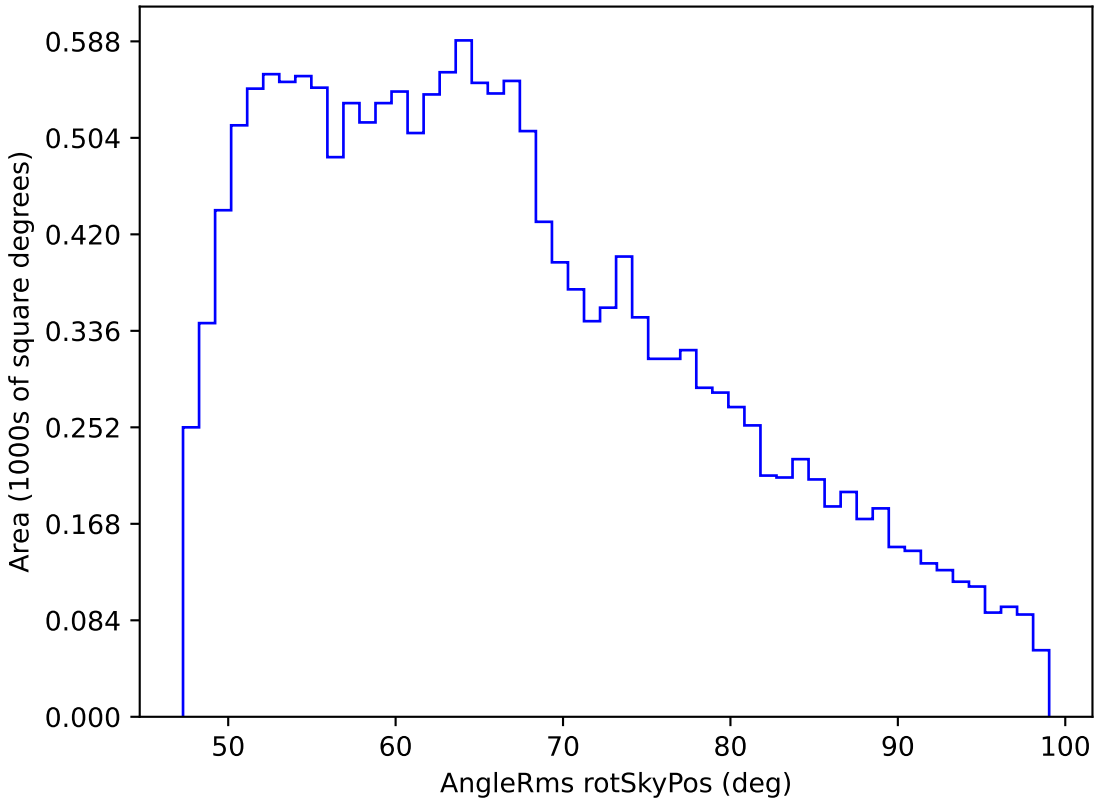
roll_pause_mjdp365_v3.4_10yrs WFD r band: AngleRms rotSkyPos
