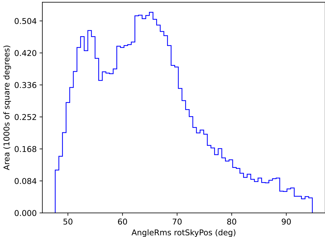
roll_pause_mjdp365_v3.4_10yrs WFD i band: AngleRms rotSkyPos
