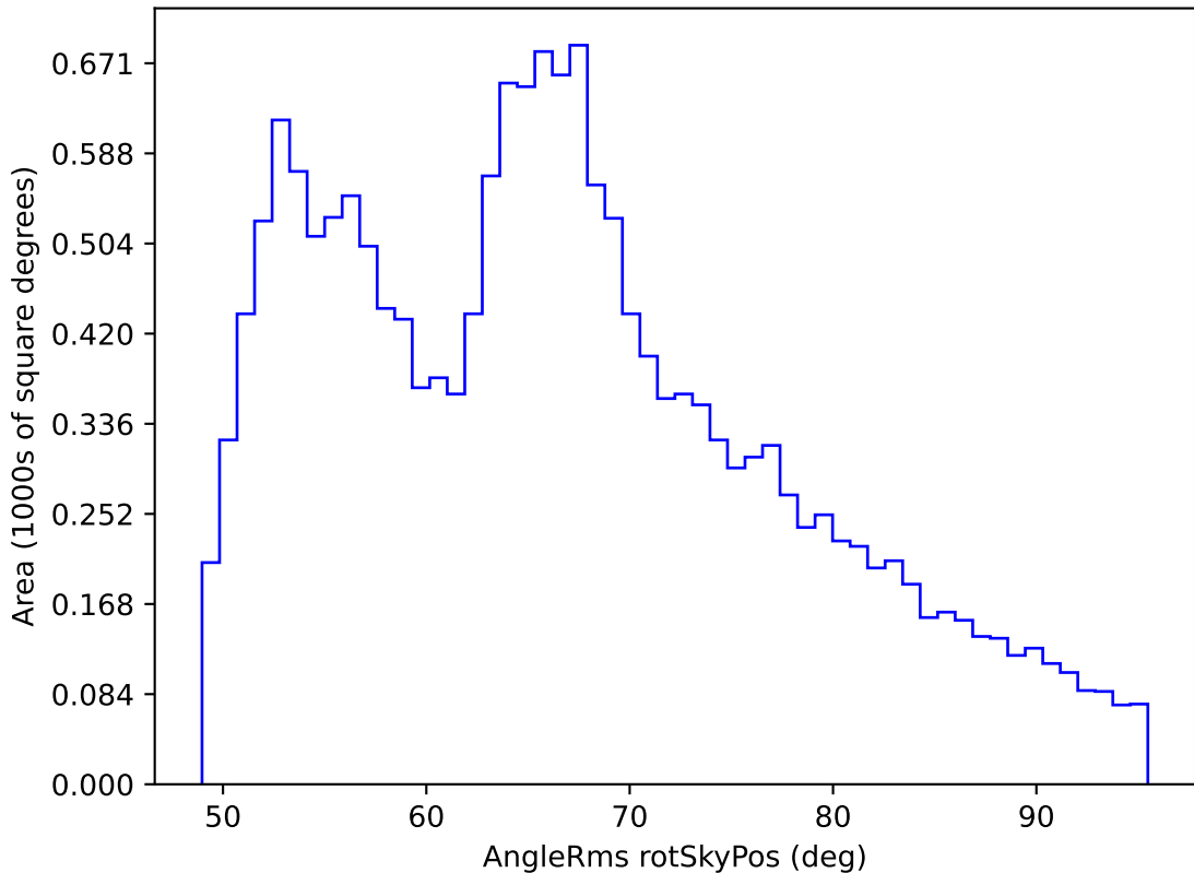
roll_pause_mjdp365_v3.4_10yrs WFD all bands: AngleRms rotSkyPos
