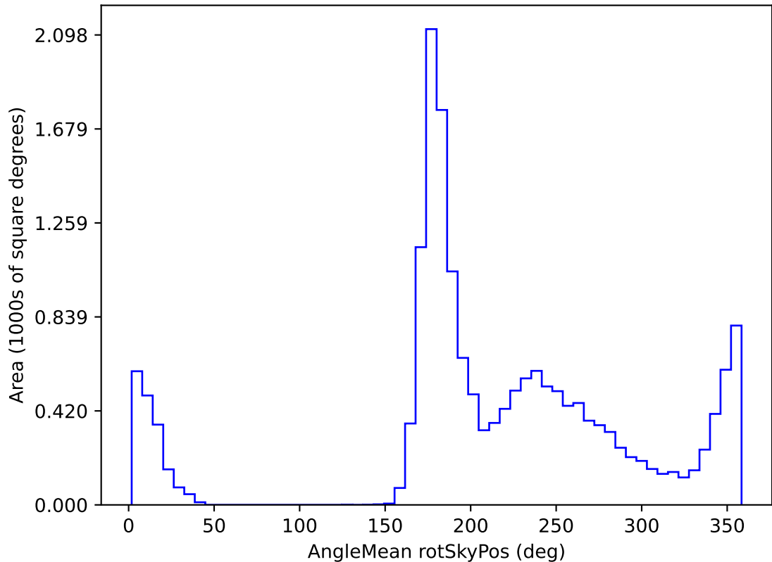
roll_pause_mjdp365_v3.4_10yrs WFD i band: AngleMean rotSkyPos
