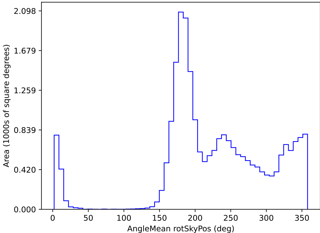
roll_pause_mjdp365_v3.4_10yrs All sky y band: AngleMean rotSkyPos
