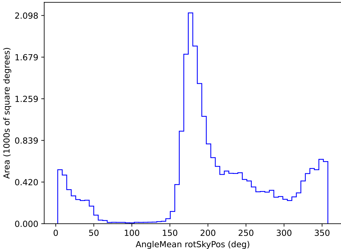
roll_pause_mjdp365_v3.4_10yrs All sky u band: AngleMean rotSkyPos
